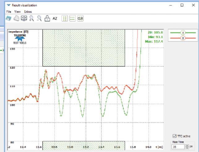
Less than 3 mm resolution on FR4 can show the effect of blind vias (red) vs. true vias (green)
