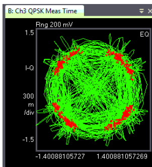
Figure 1. QPSK signal with emulated phase noise
