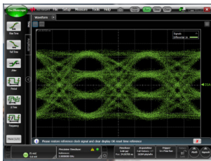
Figure 2. PAM-4 signal at 56 GBaud
